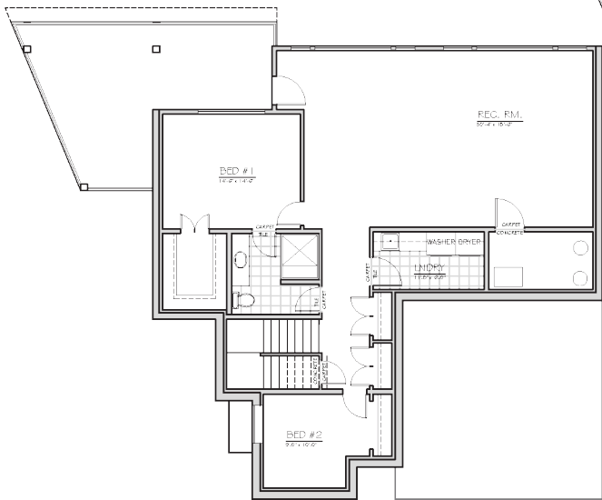
BASEMENT FLOOR LIVING - 1,582.0 sq. ft.
